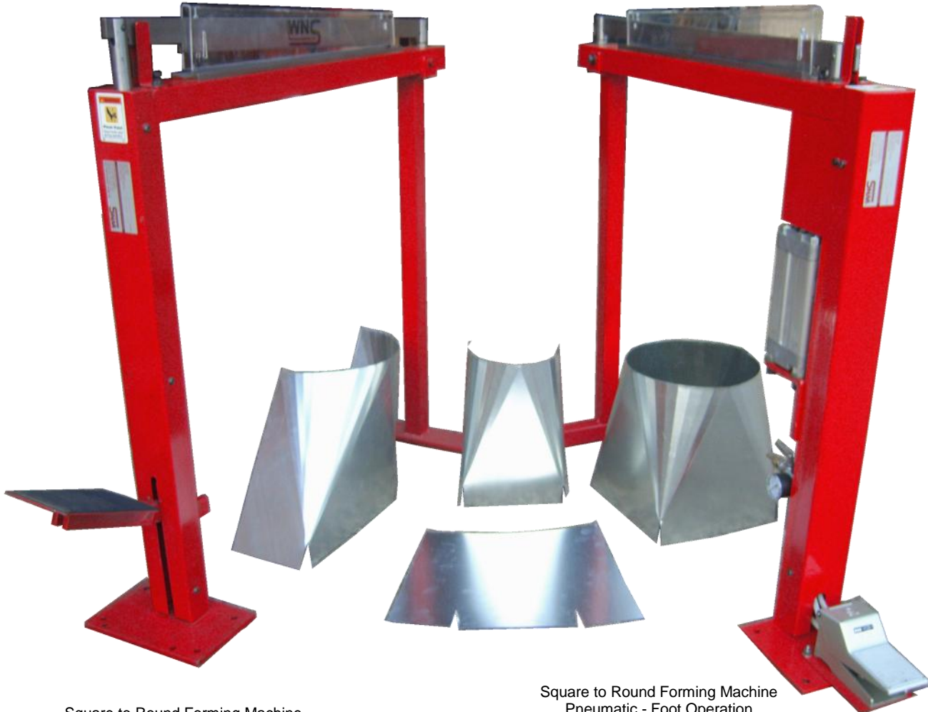
Square to Round Forming Machine Manual - Foot Operation (SR20F)
